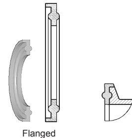
Flanged
