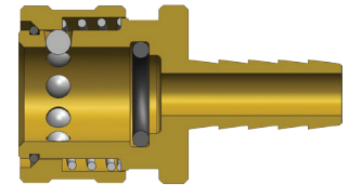
Hose Barb
