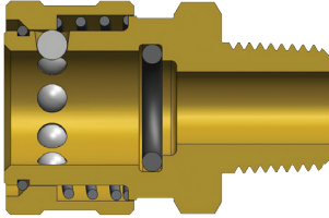
Male Thread
