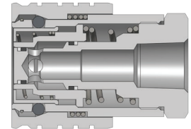
Female Thread
