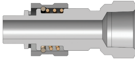
Female Thread
