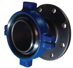
male adaptor x flange with hammer union nut
