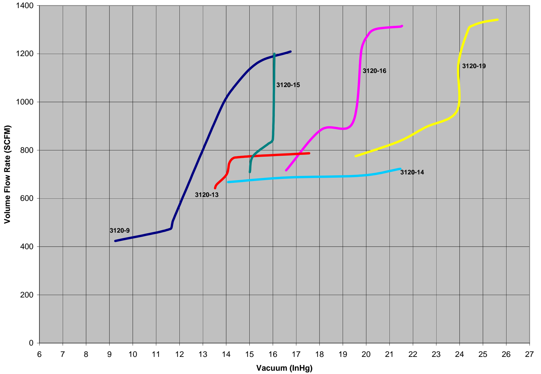
3120 Vacuum Relief Valve - Flow Rate Vs Vacuum
