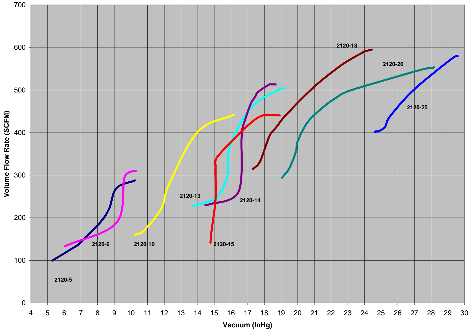
2120 Vacuum Relief Valve - Flow Rate Vs Vacuum
